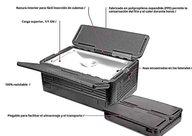
CAJA ISOTÉRMICA PLEGABLE 60X41X25 CM INT. 53.8X33.8X20CM 66066: 30,00€
